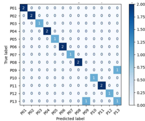
Figure 5. Confusion Matrix Sistem
