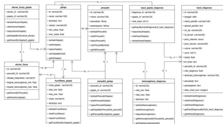
Figure 3. Class Diagram
