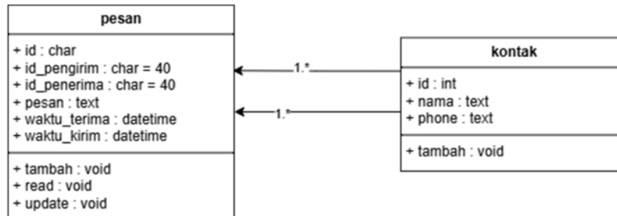
Gambar 5. Class Diagram
