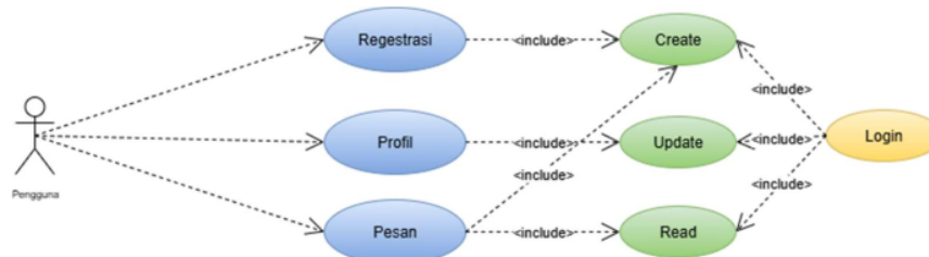
Gambar 1. Use Case Diagram
