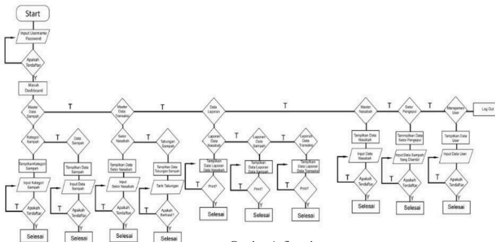
Gambar 1. flowchart
