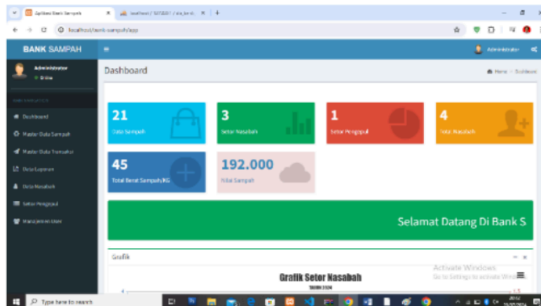
Gambar 3. Halaman Dashboard
